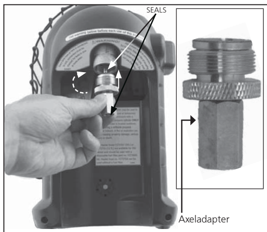
Figur 4: "Butanadapter"
