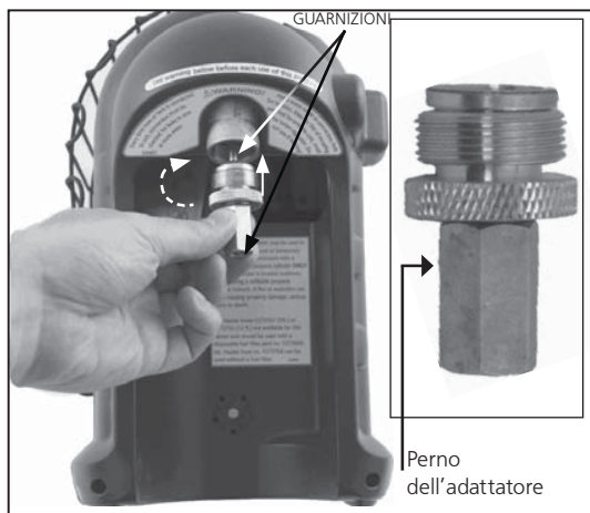
Figure 4: "butane Adapter"
